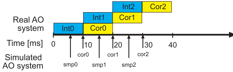
Figure 2. Scheme of the temporal delay implemented in the simulation code. The correction made on the NGS measurements is delayed by an half of the integration time. A real AO control loop is sketched for comparison, the reconstruction time is supposed to be negligible for a system running at 100\text{Hz} .
