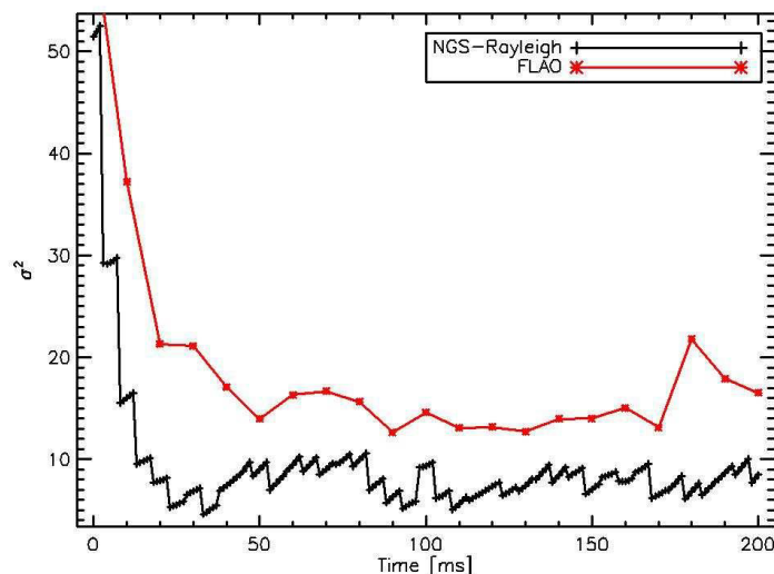
Figure 5. Variance of the residual phase in function of time at 750\text{nm} . The 2 lines refer respectively to the hybrid NGS+Rayleigh (black) and FLAO (red) systems. In the hybrid case it is visible the decorrelation of the correction of the high turbulent layers between two samples of the Pyramid WFS.
