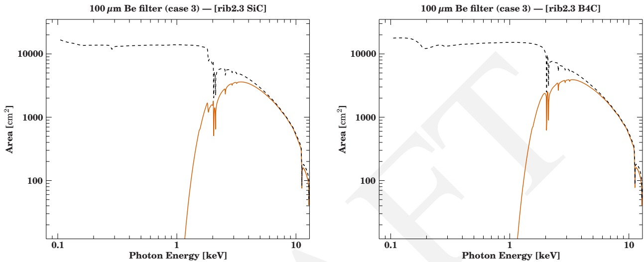
Figure 5: The final ARFs with the thick 100\ \mu\text{m} Be filter (case 3) for the two mirror configurations with Ir+SiC (left) and Ir+B4C coating (right). The dashed line indicates the nominal on-axis mirror effective area.
