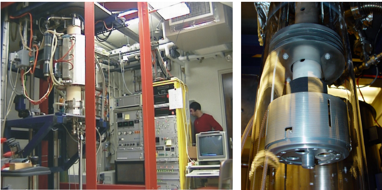
Figure 1a and 1b: Centrifuge facility (left side) and growth crucible inside the \text{SiO}_2 reactor
