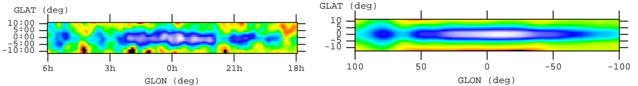
Fig. 3. Two plausible sky distribution models adopted for diffuse ^{60}\text{Fe} emission from the Galaxy. Both have been derived from COMPTEL ^{26}\text{Al} measurements (Plüschke et al., 2001; Knödseder et al., 1999). The image obtained with the Maximum-entropy method (left) shows more structure, while the image derived with the Multi-resolution Expectation Maximization Method (MREM) appears smooth from its noise-filtering, accepting only image structure which is enforced by the measurements.
