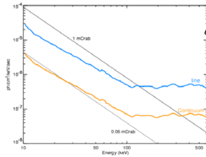
Fig. 1 [Left] The “reference design” of EXIST, with three Tungsten coded-mask imaging telescopes ( 2.7 \text{ m}^2 of CZT per telescope). Fig. 2. [Right] Sensitivity estimate ( 5\sigma , 1yr survey) based on an exposure time of 10^7 \text{ s} , allowing for 20% source duty cycle. Estimates of the continuum sensitivity assume \Delta E/E = 1 , and for lines \Delta E/E = 0.01 . The actual FWHM energy resolution below 150 keV will be less than 1 keV. Above 150 keV, Compton events will reduce the resolution.
