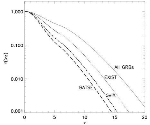
Fig. 3. Predicted fraction of GRBs with red shift greater than z .
