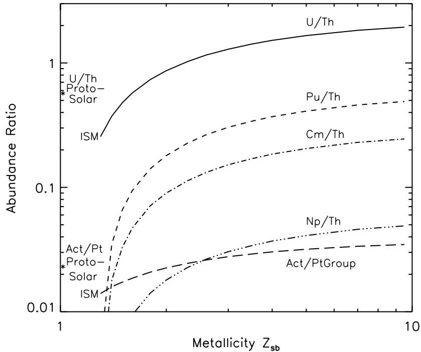
Fig. 2. Expected cosmic-ray actinide abundance ratios as a function of superbubble core metallicity. Also indicated are the estimated U/Th and Actinide/Pt-Group ( Z = 75 to 79 ) ratios in the current interstellar medium (ISM) and in the SN-enriched proto-solar material.
