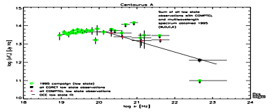
Fig. 5: Low state spectrum (all other viewing periods) and data from the multiwavelength campaign 1995
