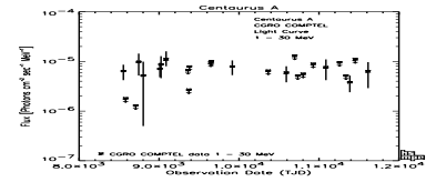
Fig. 2: All COMPTEL measurements
