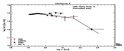
Fig. 4: Intermediate state spectrum (viewing period 12)
