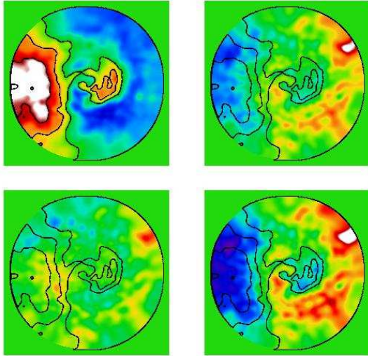
Fig. 10.— Relative deviations from azimuthally averaged values of a) surface brightness I b) temperature T c) pressure p = T\sqrt{I} and d) entropy s = T/I^{1/3} . Contours mark the regions of excess surface brightness (from the first image). The color scale is the same for all three plots (from -0.5 to +0.5, see color bar in Fig.7). Clearly the azimuthal variations in pressure are smaller than in any other quantity.
