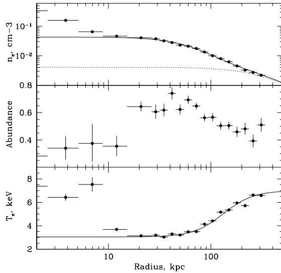
Fig. 8.— Radial profiles of deprojected parameters. The parameters were obtained using a single temperature APEC model with fixed low energy absorption fitted to deprojected spectra for a set of spherical shells centered at NGC 1275. The data points in the innermost region ( \sim 10 kpc) are affected by the presence of the bright compact source – the nucleus of NGC 1275. Analytical approximations for the density and temperature are shown as solid lines (see text).
