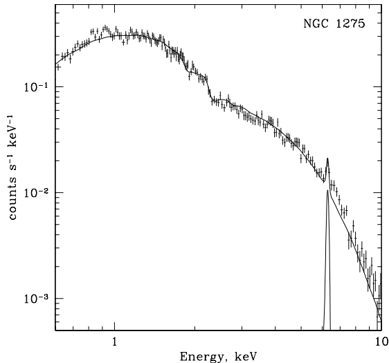
Fig. 5.— NGC 1275 spectrum determined as the difference between the spectra extracted from the 14'' (radius) circle and the annulus from 14'' to 28''. The position of the line is consistent with the neutral iron fluorescent line at 6.4 keV with the redshift of 0.0176.
