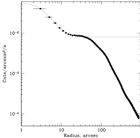
Fig. 4.— Radial dependence of the surface brightness in the 0.3–5 keV band. The dotted line shows the sum of the telescope Point Spread Function (PSF) plus a constant, illustrating that the central excess is consistent with being due to the NGC 1275 nucleus contribution.
