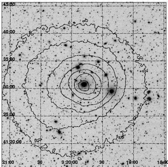
Fig. 1.— Surface brightness contours in the 0.3–5 keV energy range (corrected for the background and telescope vignetting) superposed onto a DSS optical image ( 30' \times 30' ). The X-ray image has been smoothed with an 8'' Gaussian. The central galaxy is NGC 1275. A chain of bright galaxies is visible to the West.
