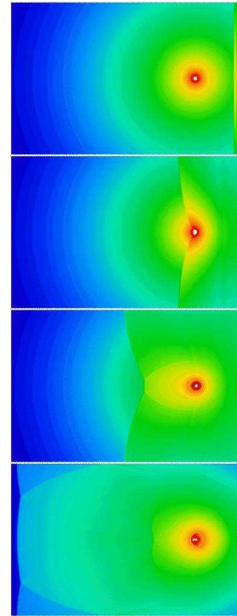
Fig. 11.— Snapshots of the gas density at 0, 0.3, 0.7, 1.6 Gyr from the beginning of the simulations. The box shown is 4 \times 6 Mpc. The density, temperature and velocity of the gas in a narrow slab on the right side of the box were set to mimic the impact of a piston which is first driven into the gas at the Mach number of 2 and then suddenly stopped.
