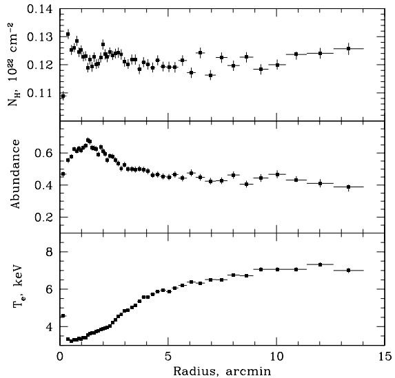
Fig. 6.— Radial profiles of N_H , T_e and heavy element abundance calculated for a set of annuli centered at NGC 1275. The parameters were obtained using a single temperature APEC model. The first two data points in the innermost region are affected by the presence of the bright compact source – the nucleus of NGC 1275.
