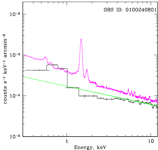
Fig. 3.— The same as in the previous figure but for the observation performed \sim 14 hours after the end of the Perseus observation. The background level was still enhanced compared to the quiescent state, although a factor of \sim 2 lower than in the Perseus observation. The upper curve shows the quiescent background spectrum. The histogram is the spectrum accumulated over the 8' - 13.75' annulus and corrected for the quiescent background. The power law shows the predicted “flare” background component, obtained with the same procedure as was used for the Perseus observation.
