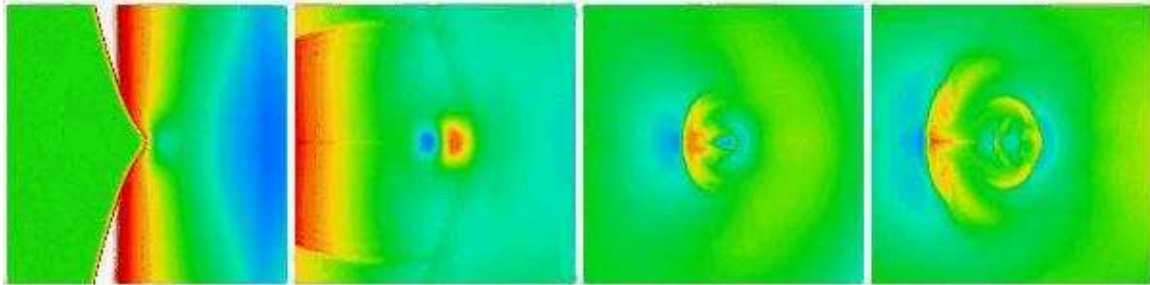
Fig. 12.— Relative deviation of the gas density from the initial value (blue color marks the regions with the density below the initial value while yellow and red correspond to overdense regions). The box shown is approximately 2 Mpc on a side. The snapshots are taken at 0.3, 0.7, 2.3, 3.9 Gyr from the beginning of the simulation.
