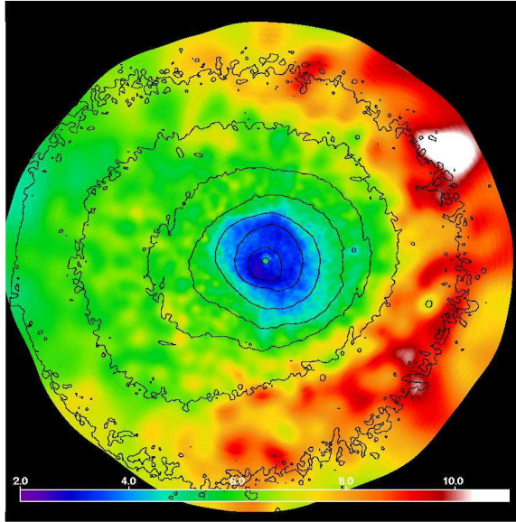
Fig. 9.— Gas temperature map ( 30' \times 30' ). The temperature is derived from adaptively smoothed data with an effective number of counts within each smoothing window of \sim 10^4 . Contours show the surface brightness distribution.
