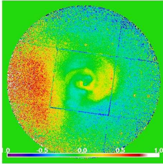
Fig. 7.— Relative deviation of the surface brightness from the azimuthally averaged value. The image shown is 30' \times 30' . Clearly seen are: the region of excess emission to the East from the center, an edge-like structure 5' - 7' to the West from the center and complicated structure in the inner 1' - 2' region.
