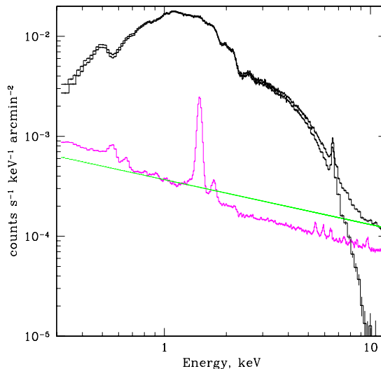
Fig. 2.— The spectrum of the 8' - 13.75' annulus around NGC 1275 and the background spectrum. Two lower curves show the blank field “quiescent” background and the additional “flare” background component (power law) assumed in the analysis. Two upper curves show the source spectrum with the quiescent background subtracted (upper curve) and the source spectrum with both the quiescent and flare background components subtracted (lower thick curve). The normalization of the flare background has been estimated using the data above \sim 11 keV.
