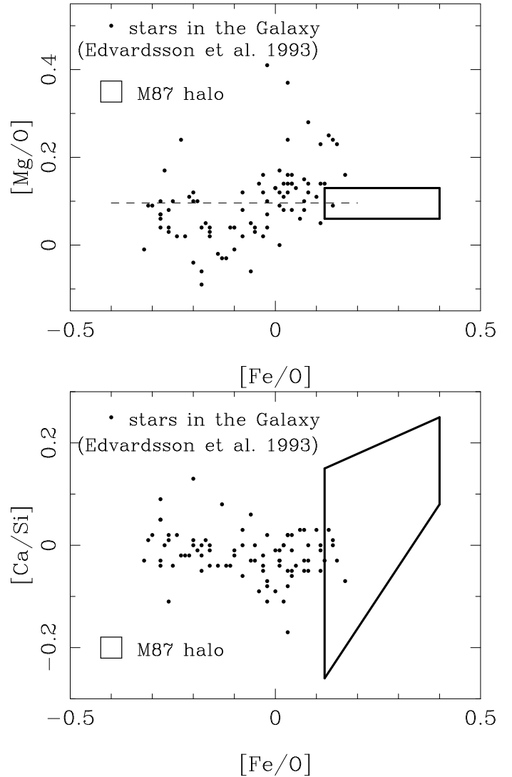
Fig. 18. [\text{Mg}/\text{O}] , and [\text{Ca}/\text{Si}] are plotted against [\text{Fe}/\text{O}] . Those of disk stars (Edvardsson et al. 1993; closed circles) in the Galaxy are also plotted.
