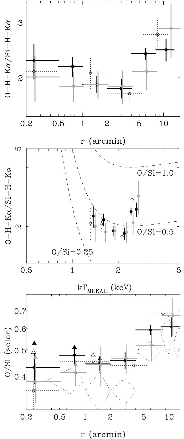
Fig. 7. The line ratios of K\alpha lines of H-like O and Si of the EMOS (black) and the EPN (gray), plotted against the radius (upper panel) and the best fit temperature fitted with the single MEKAL model (middle panel). Solid and dotted data correspond to projected and deprojected data, respectively. Dashed lines in the middle panel correspond to constant abundance ratios in unit of the solar ratio. The derived abundance ratios are plotted in the bottom panel. Within 2 arcmin, contributions of the lower temperature component are considered. Triangles are the best fit values of the abundance ratio, assuming the temperature is larger than 1.7 keV. The diamonds correspond to the abundance ratios derived from the deprojected EMOS spectra using the MEKAL model fit. Errors represent the
