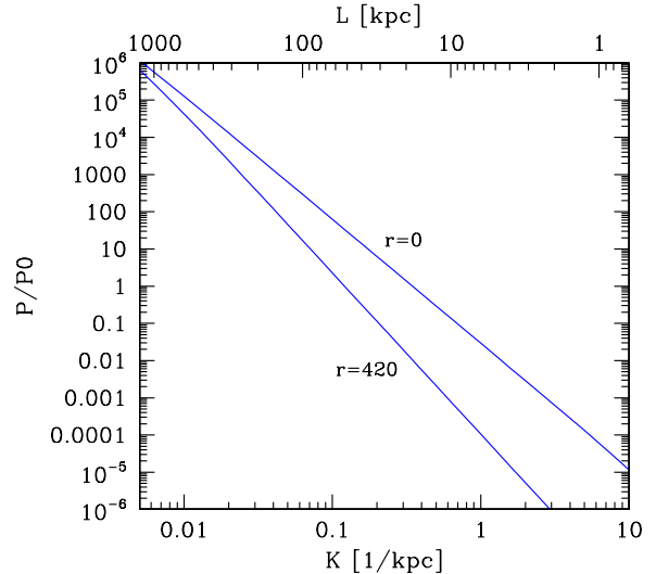
Fig. 2. Pressure power spectra with an intrinsic slope of n = -7/3 as expected for a Kolmogorov/Oboukhov turbulence ( r = 0 ) and its projection (420 kpc) as seen along the LOS through the center of a cluster with a core radius of r_c = 420 kpc and a slope parameter of \beta = 0.75 as measured for the Coma cluster. In order to illustrate the projection effects over a large scale range we did not introduce any characteristic scale which limits the spectra at large and small scales.
