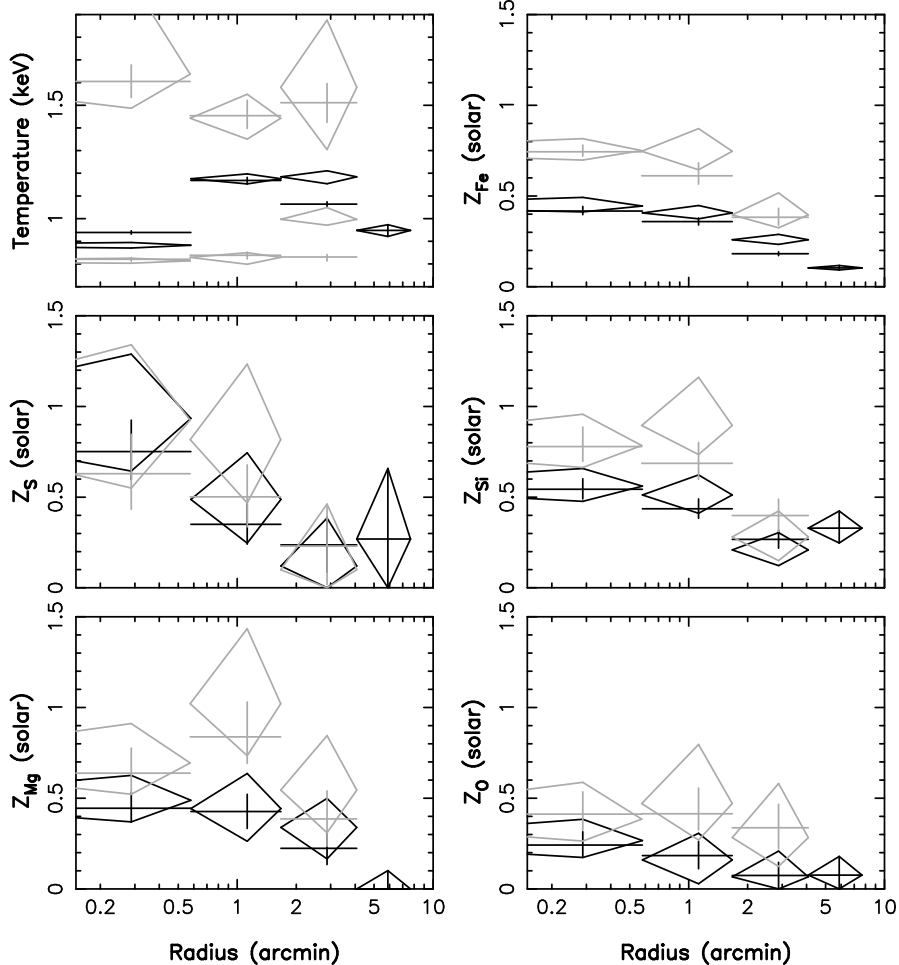
Fig. 2. The deprojected (diamonds) and projected (crosses) temperature and abundance profiles and 1\sigma errors for the 1T (black) and 2T (gray) models. The emission measures of the hot and cool components of the 2T model are displayed in Figure 6.
