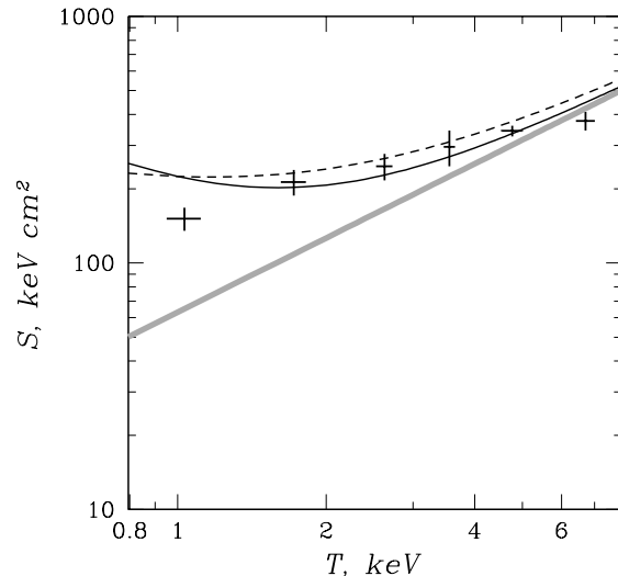
FIG. 3.— Scaling relation between entropy ( S ), measured at 0.1 R 200 , and temperature ( T ). The solid black line is the inferred relation accounting for a constant energy excess injected by radio galaxies (see text for details). The grey line is the expected self-similar relation. The points show the binned means from the observations by Ponman et al. (2003). The dashed line is the same as the solid line but considering the self-similar scaling M_{\text{gas}} \propto T^{1.5} .
