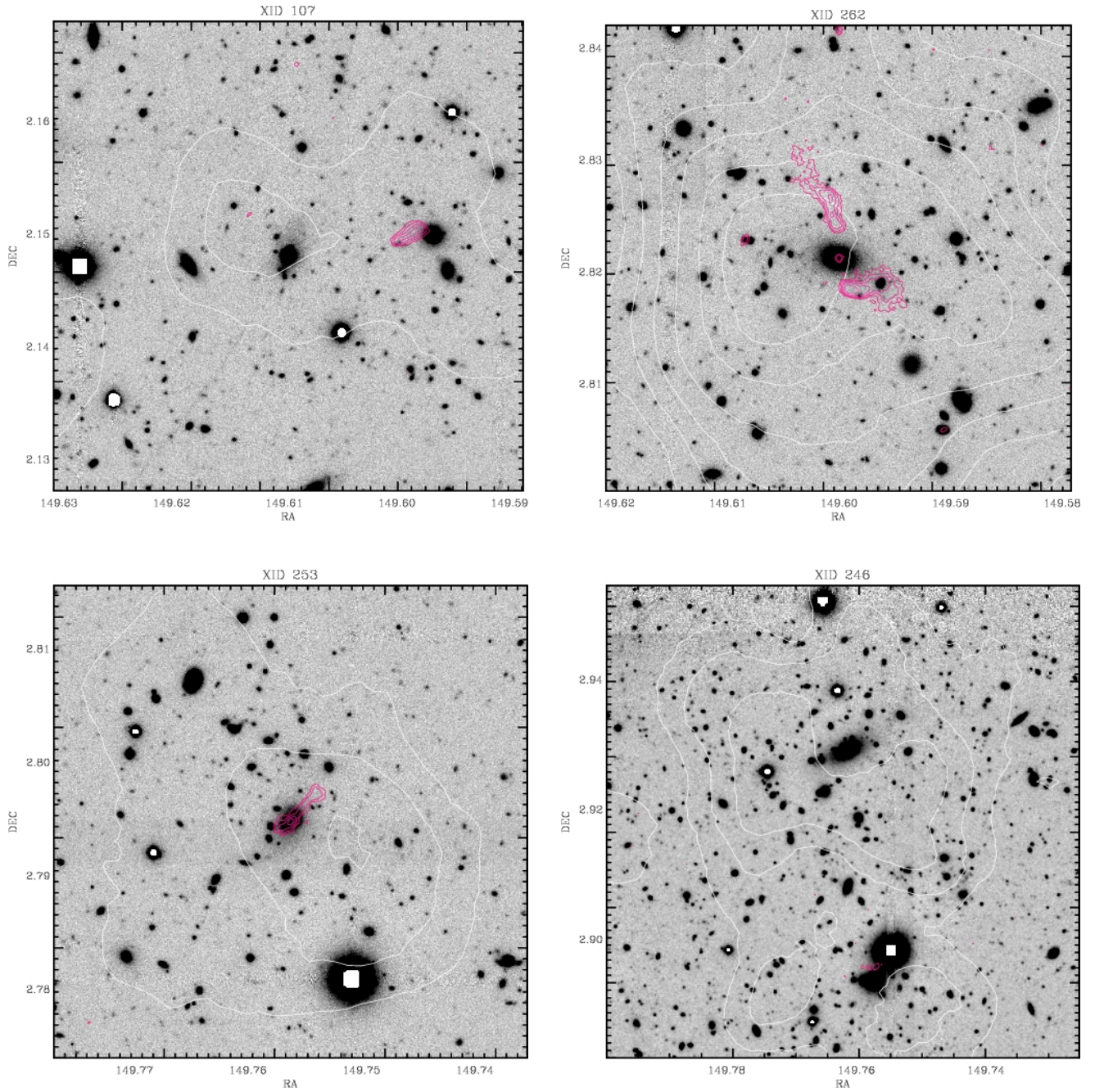
FIG. A1.— Figure A1 presents the contours maps of the radio 20 cm emission (magenta lines) superimposed to the SUBARU z_p band image for each of the groups listed in Table 1. Images are 3 \times 3 arcmin and centered on the group center, except XID246 which is 4 \times 4 arcmin wide and offset from the center group because of its location on the edge of the SUBARU field coverage. The white line shows the contours of X-ray flux significance. The contours correspond to [3, 6, 9, 12, 15, 18, 21, 24] \sigma X-ray flux significance.
