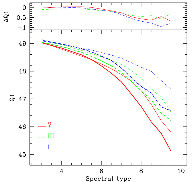
Fig. 15. Same as Fig. 14 but for He I ionising fluxes.
