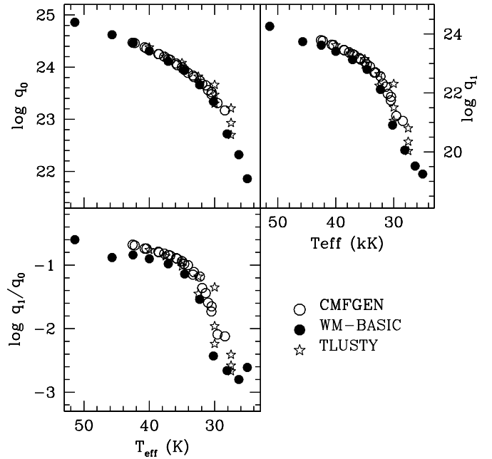
Fig. 17. Same as Fig. 16 for supergiants.
