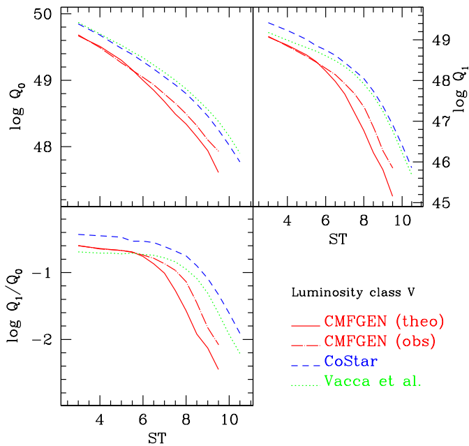
Fig. 18. Comparison between the present ionising fluxes of dwarfs and the results of Vacca et al. 1996 and Schaerer & de Koter (1997, CoStar models).
