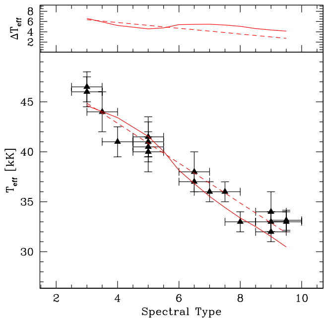
Fig. 4. Effective temperature scale for dwarfs as derived from our model grid (“theoretical” scale, solid line) compared to “observational” results based on non-LTE line blanketed models including winds (Herrero et al. 2002, Repolust et al. 2004 and Martins et al. 2005). The dashed line is the result of linear regression to the data points. The typical error bars for the observational results are \pm 0.5 unit for spectral types and are taken from detailed spectroscopic analysis for T_{\text{eff}} . The upper panel shows the difference between the relation of Vacca et al. (1996) and our T_{\text{eff}} scales (solid line: relation from model grid; dashed line: relation from spectroscopic analysis).
