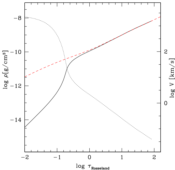
Fig. 1. Typical hydrodynamical structure: density as a function of Rosseland optical depth for a model with T_{\text{eff}} = 40000 K, \log g = 3.50 and \dot{M} = 1.410^{-5} M_{\odot}/\text{yr} . The red dashed line is the initial TLUSTY structure on which a \beta velocity law is connected to give the final CMFGEN input structure (black solid line). The dotted line shows the CMFGEN velocity structure as a function of Rosseland optical depth. The TLUSTY and CMFGEN structures are similar in the very inner atmosphere and start to depart from each other around \log \tau_{\text{Rosseland}} \sim 0 which corresponds to a velocity of a few \text{km s}^{-1} .
