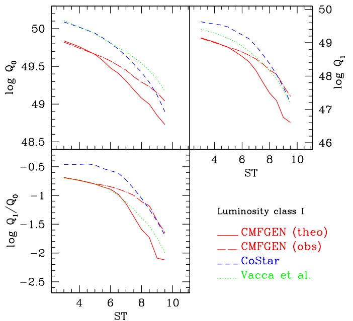
Fig. 20. Same as Fig. 18 for supergiants.
