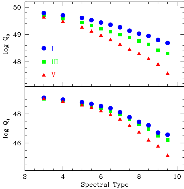
Fig. 13. Ionising fluxes as a function of spectral type for dwarfs (triangles), giants (squares) and supergiants (circles) derived using the theoretical T_{\text{eff}} scale.
