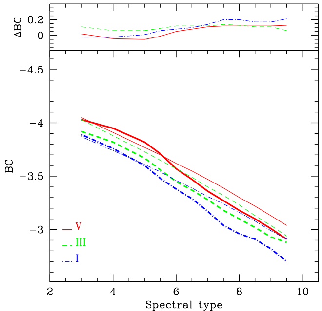
Fig. 11. Same as Fig. 10 but with the bolometric corrections derived using the “theoretical” (bold lines) and “observational” (thin lines) T_{\text{eff}} scales. The upper panel shows the differences between “theoretical” and “observational” BCs.
