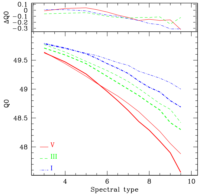
Fig. 14. Lyman continuum photon fluxes derived using the theoretical (bold lines) and observational (thin lines) T_{\text{eff}} scales. Solid lines are for dwarfs, dashed lines for giants and dot-dashed lines for supergiants. The upper panel shows the difference between theoretical and observational results.
