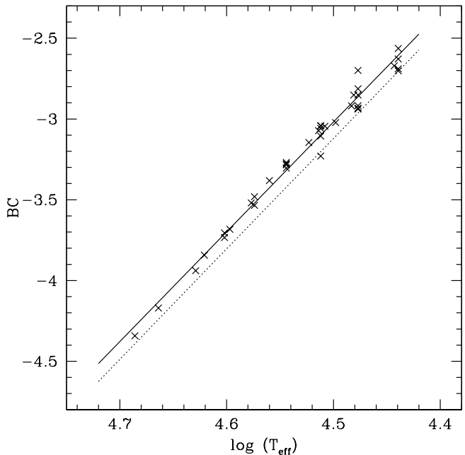
Fig. 9. Bolometric correction as a function of effective temperature from our set of CMFGEN models. The solid line is the linear regression (Eq. 4) and the dotted line is the relation of Vacca et al. (1996) and is shifted by \sim 0.1 mag compared to our relation.
