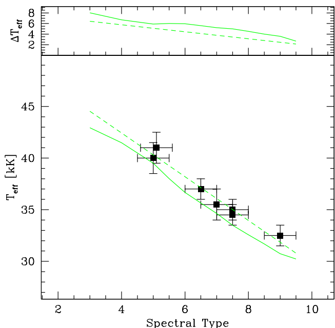
Fig. 5. Same as Fig. 4 for giants.
