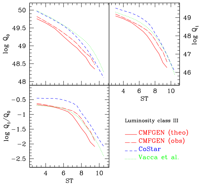
Fig. 19. Same as Fig. 18 for giants.
