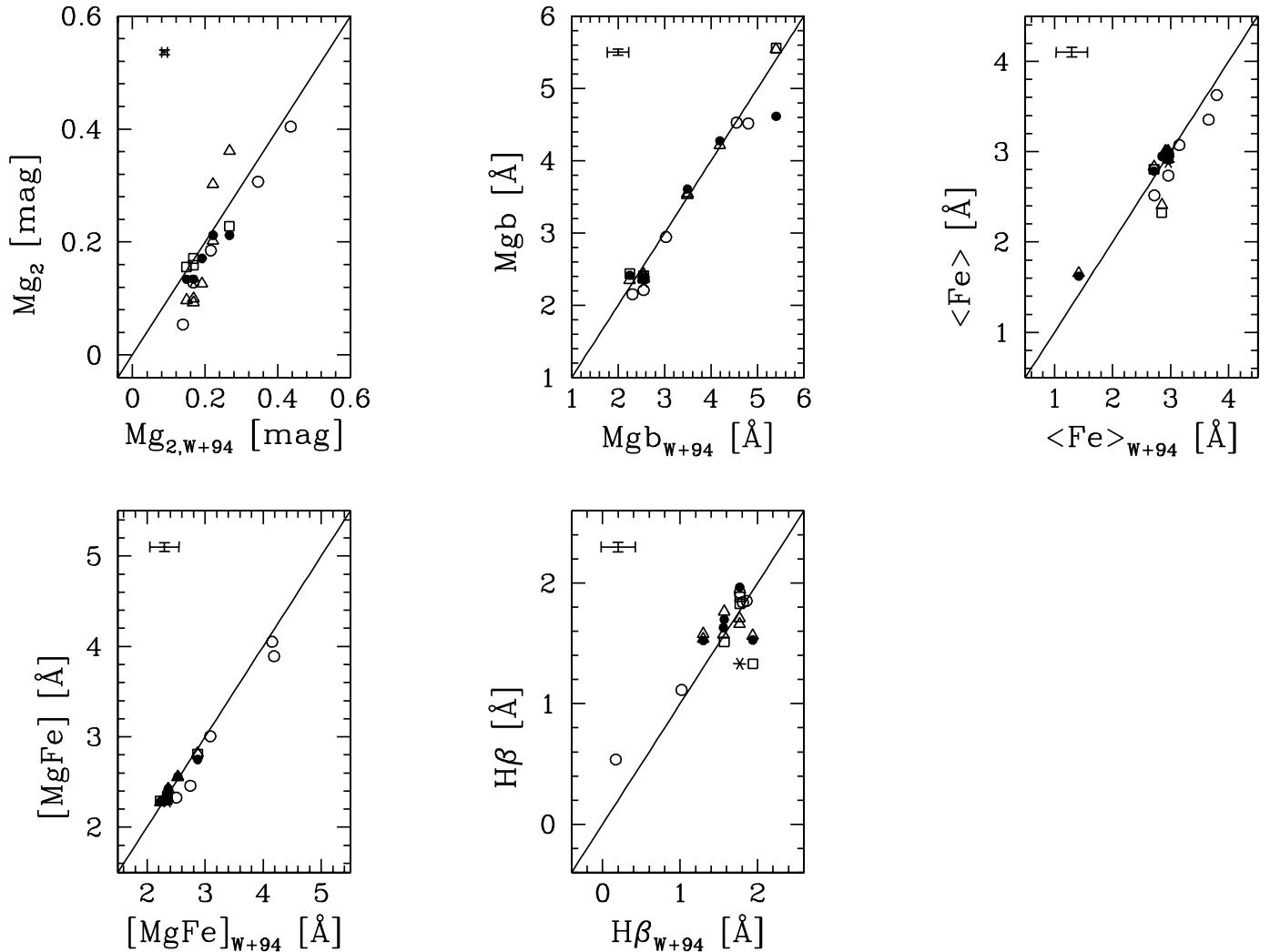
FIG. 6.— Comparison of the values for the line strength indices of Mg_2 , Mg\ b , Mg_2 , \langle Fe \rangle , [MgFe] , and H\beta measured for a sample of stars in this work and in Worthey et al. (1994) W+94. The open circles, filled circles, squares, asterisks, and triangles refer to data obtained in runs 1, 2, 3, 4, and 5, respectively. In each panel the error bars in the upper left corner indicate the mean errors, and the solid line shows the line of correspondence.
