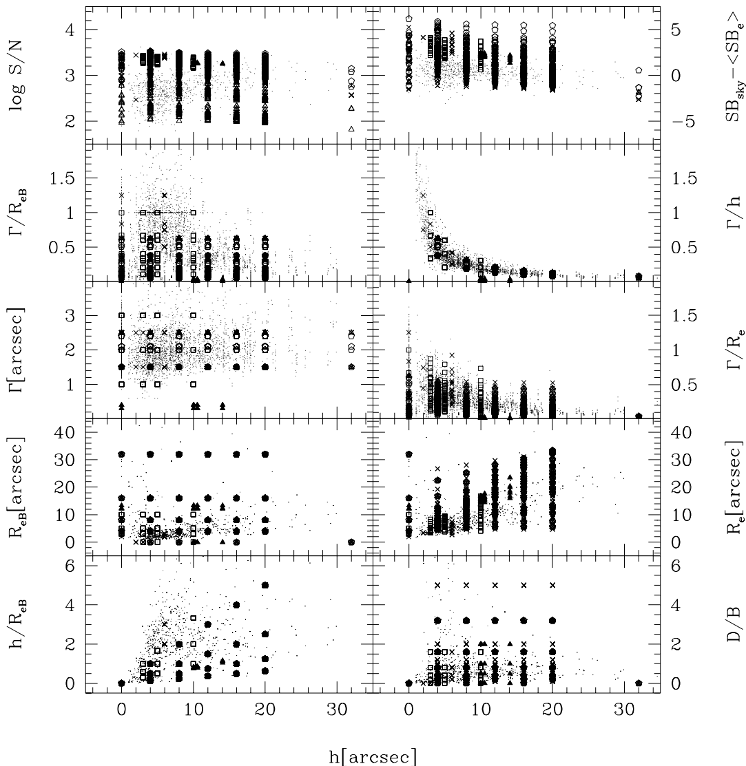
FIG. 1.—Parameter space of the R^{1/4} plus exponential profile of the Monte Carlo simulations discussed in Figs. 2–11. Crosses , models of Figs. 2–7 (see also Table 2). Filled triangles , models of Fig. 8. Open triangles , models of Fig. 9. Open squares , models of Figs. 10–11. Open pentagons , models of Fig. 12. Open hexagons , models of Fig. 13. The small dots show the position of the EFAR galaxies as determined in Paper III. The parameters of bulge-only models are shown with h = 0 . The parameters of disk-only models are shown at R_{eB} = 0 . See discussion in § 3.
