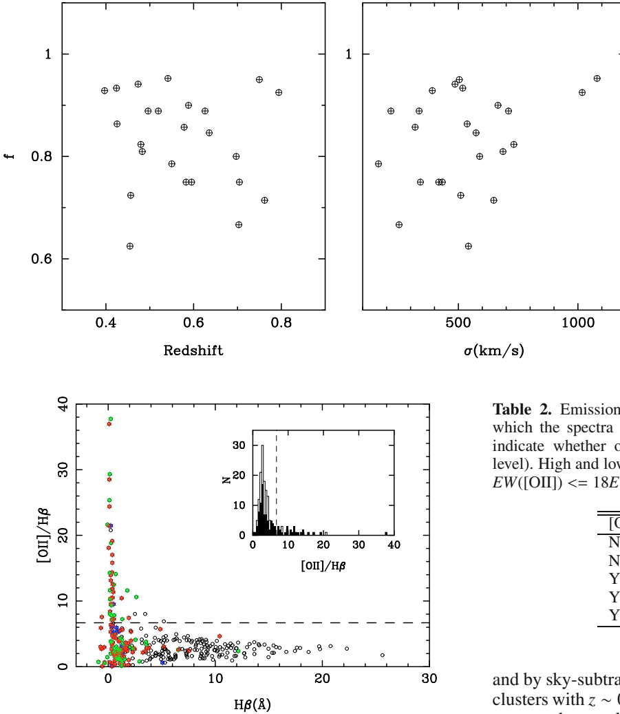
Fig. 4. Ratio between [\text{OII}] and \text{H}\beta for the full EDisCS sample of cluster members (black dots). Red, green, and blue stars indicate the red-sequence galaxies in the 0.45, 0.55, and 0.75 redshift bins, respectively. The [\text{OII}]/\text{H}\beta distribution is also presented in the form of a histogram: the black-filled zone represents the red-sequence galaxies, to be compared to the full sample. Dashed lines indicate the [\text{OII}]/\text{H}\beta = 6.7 limit above which the galaxy emission is considered to be due to mechanisms other than star formation.
