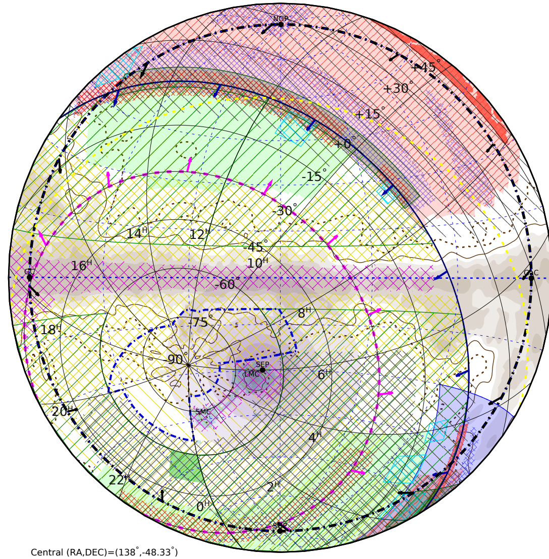
West Galactic Hemisphere
