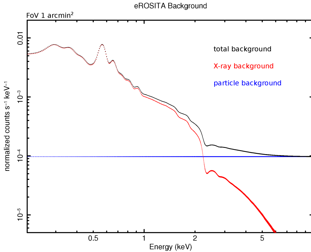
Fig. 1: eROSITA background model (plot: credit K. Borm)
