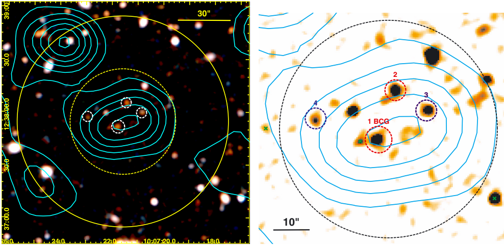
Fig. 1. Optical/NIR appearance of the galaxy cluster XMMU J1007.4+1237 at z = 1.555 with XMM-Newton X-ray contours overlaid in cyan in the logarithmically spaced range [0.014, 0.074] counts arcsec -2 (0.35–2.4 keV). Left: z + H -band color composite ( 2.3' \times 2.3' ) centered on the cluster. Spectroscopic cluster members are marked by white circles, 30'' (dashed) and 60'' (solid) radii around the X-ray center are indicated in yellow. Right: H -band zoom on the cluster core region. Red (IDs 1 and 2) and blue starburst (IDs 3 and 4) cluster members are marked by small circles, spectroscopically confirmed foreground galaxies are indicated by green crosses, and the outer dashed circle represents the 30'' radius.
