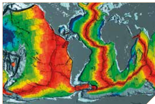
Radioactivity drives tectonic plate activity
