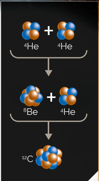
The 'burning' of helium to carbon via the 'triple alpha' process, which is responsible for the amount of carbon created in stars and needed for life. It is an unlikely reaction but is driven by subtle coincidental energy relationships between carbon, helium and beryllium nuclei
