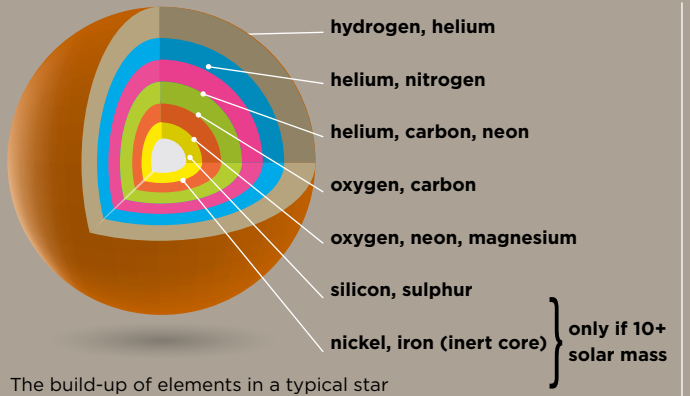
The build-up of elements in a typical star
